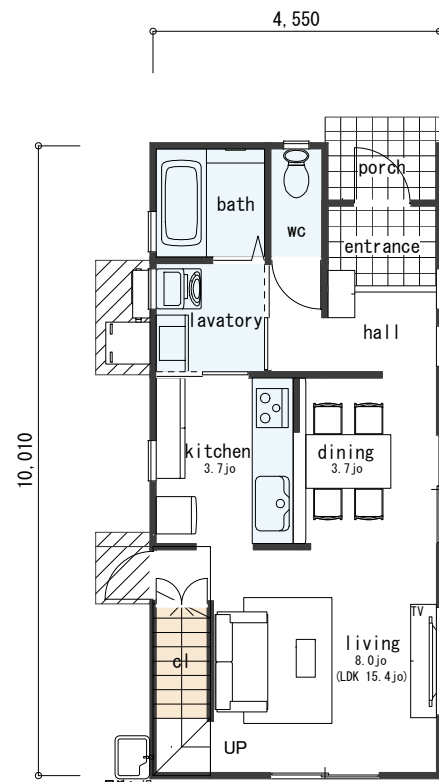
FLOOR PLAN 1F
