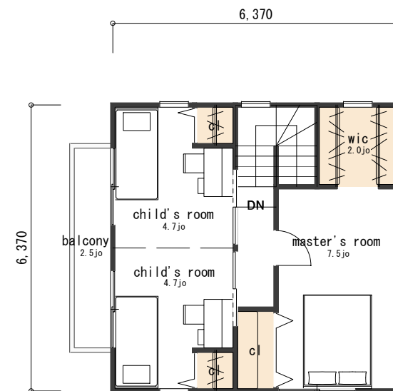
FLOOR PLAN 2F
