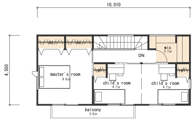
FLOOR PLAN 2F
