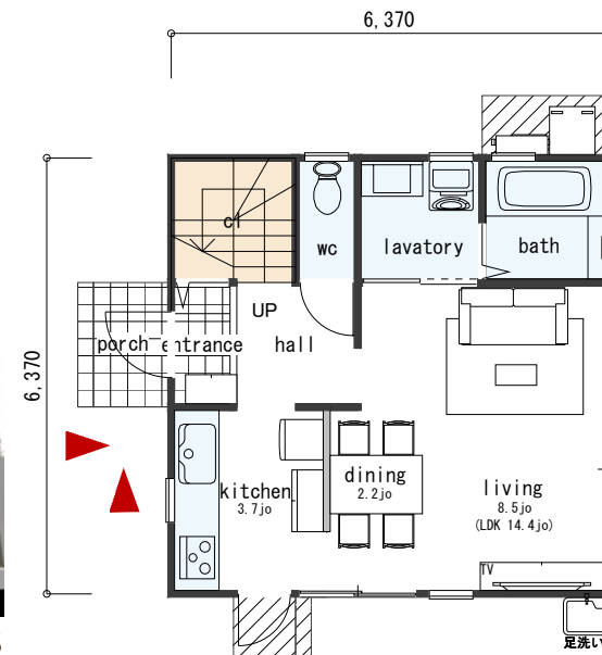
FLOOR PLAN 1F
