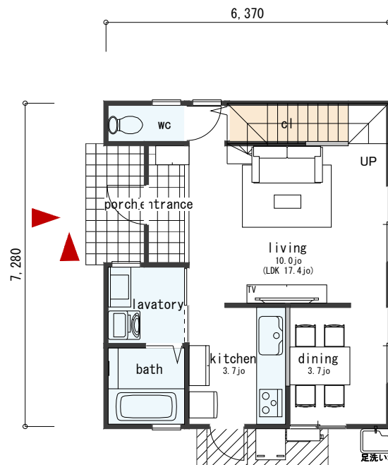
FLOOR PLAN 1F
