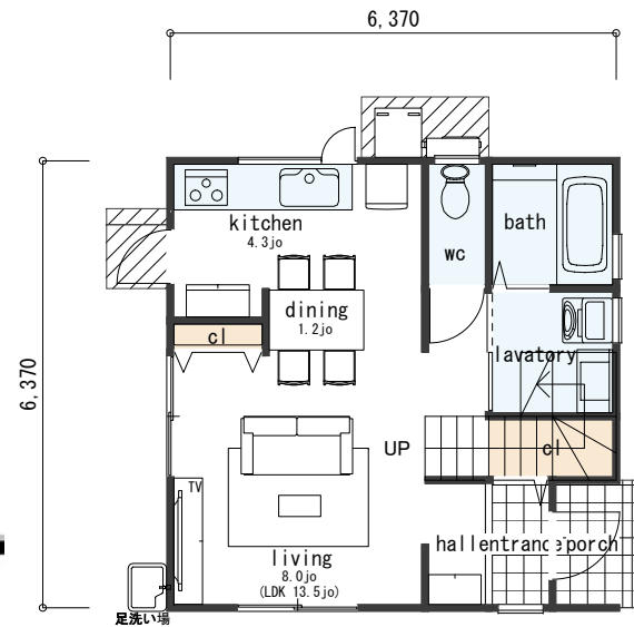
FLOOR PLAN 1F
