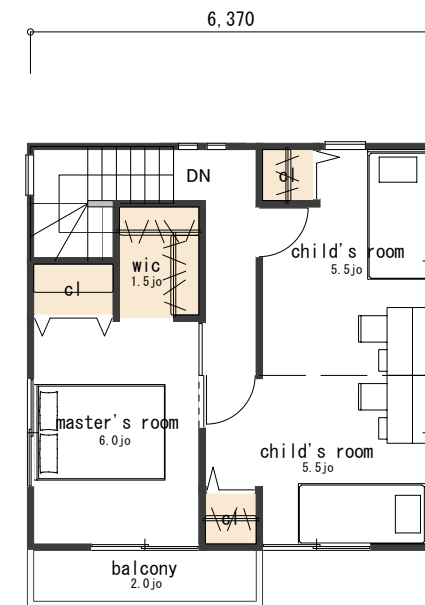
FLOOR PLAN 2F
