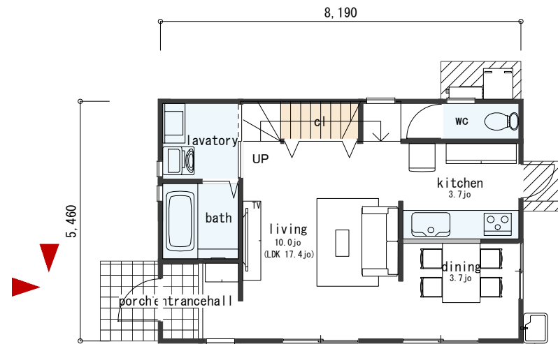
FLOOR PLAN 1F
