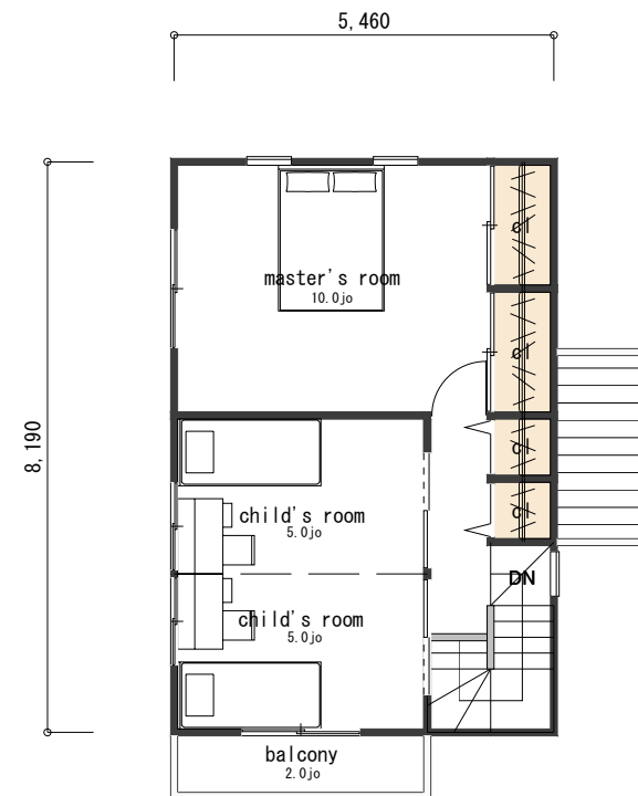
FLOOR PLAN 2F
