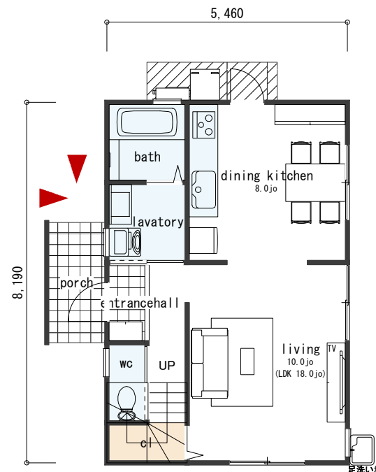
FLOOR PLAN 1F
