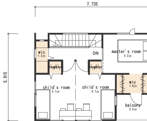
FLOOR PLAN 2F
