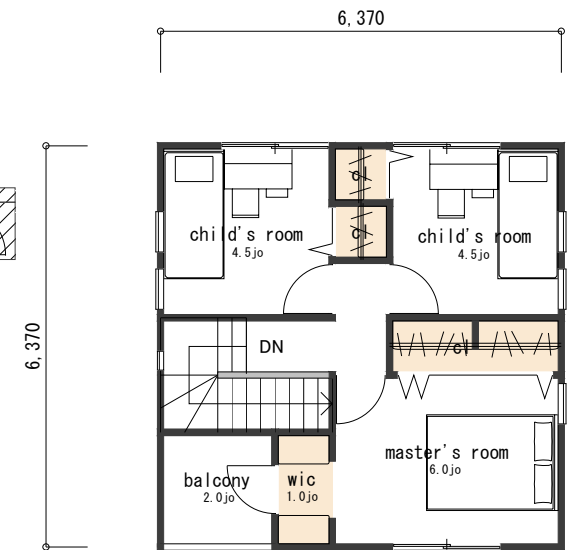
FLOOR PLAN 2F
