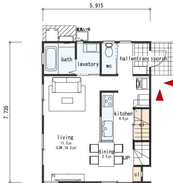
FLOOR PLAN 1F
