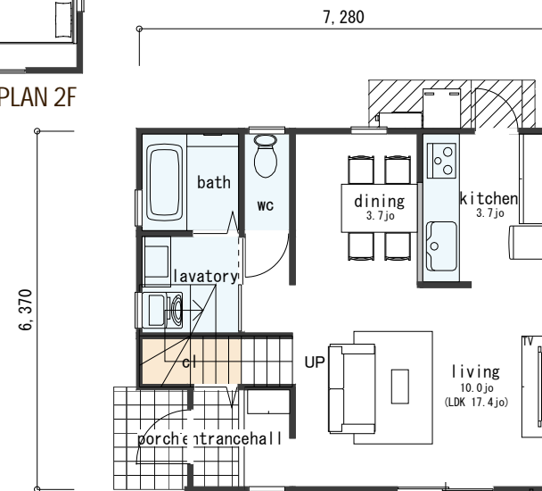
FLOOR PLAN 1F
