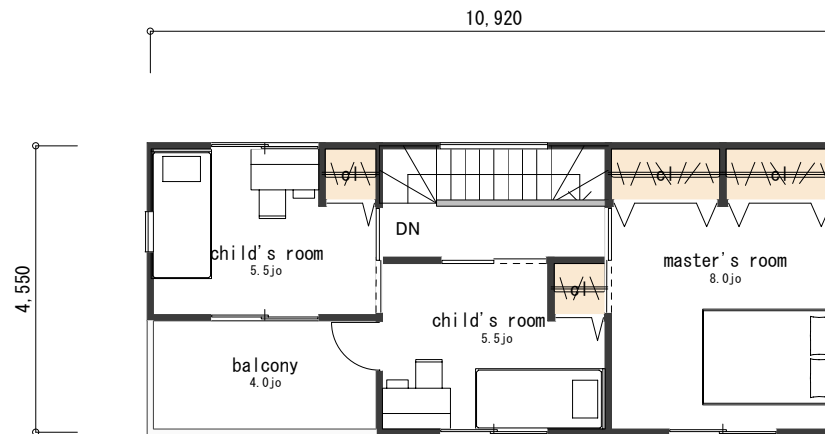
FLOOR PLAN 2F
