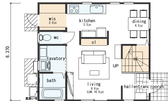
FLOOR PLAN 1F
