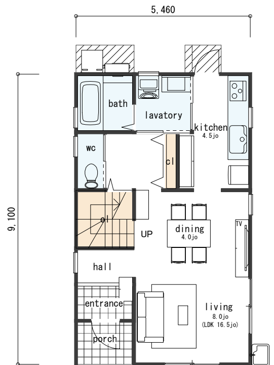
FLOOR PLAN 1F
