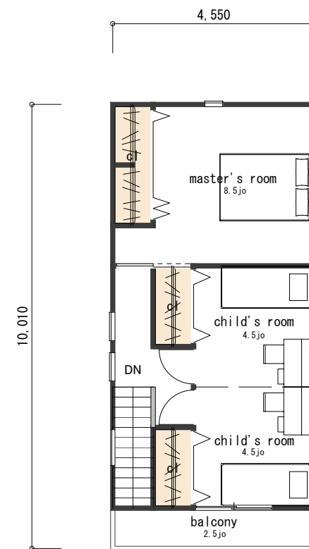
FLOOR PLAN 2F
