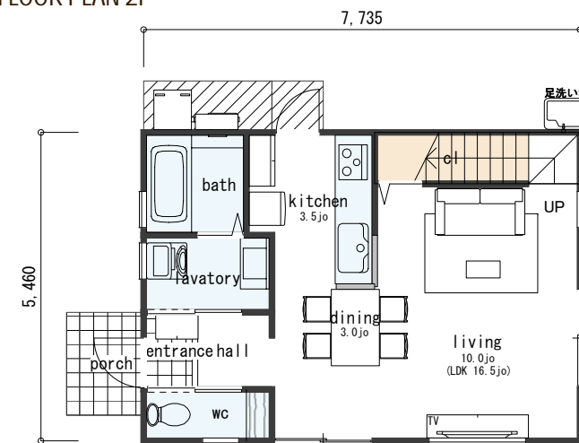
FLOOR PLAN 1F
