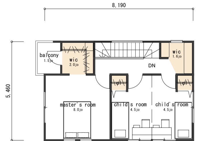
FLOOR PLAN 2F
