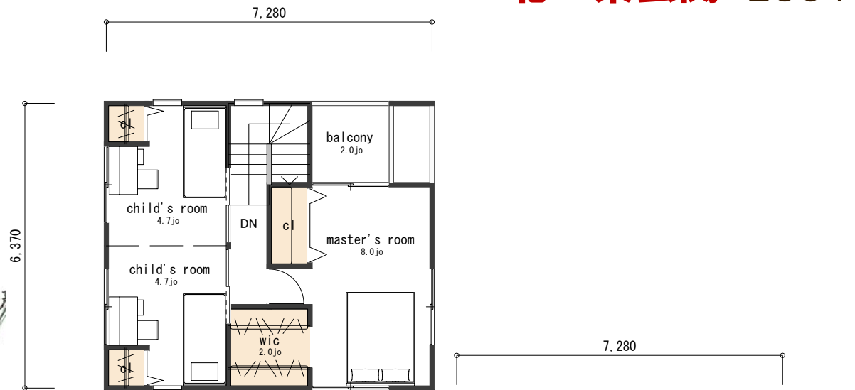
FLOOR PLAN 2F
