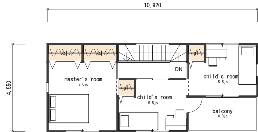
FLOOR PLAN 2F
