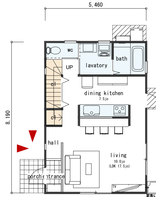
FLOOR PLAN 1F
